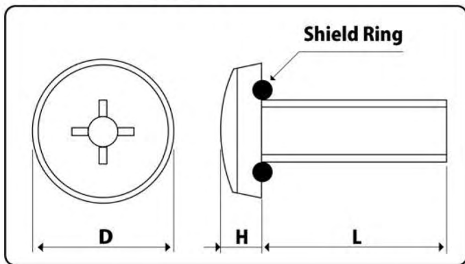
Machine Screw
